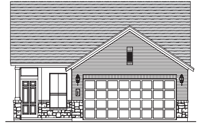
ELEVATION C
